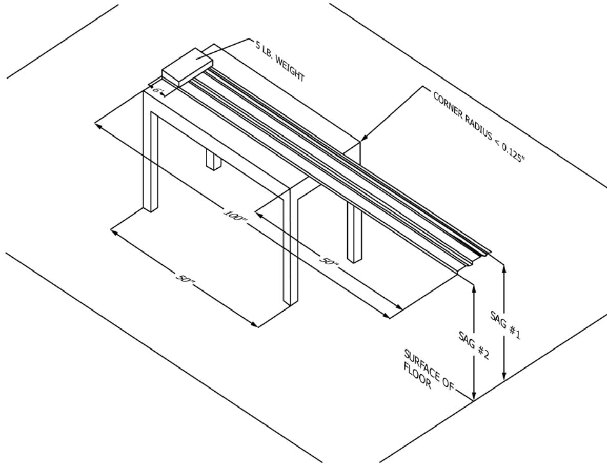
FIG. 1 Testing Apparatus for Rigidity of Vinyl Siding
