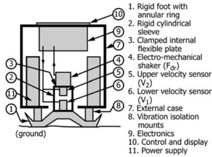
FIG. 1 Possible Apparatus Schematic
