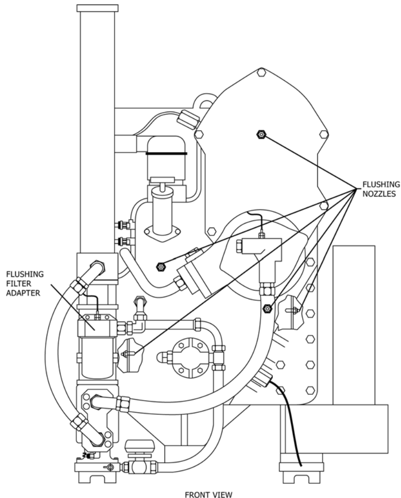
FIG. A11.1 Flushing Nozzle Locations
