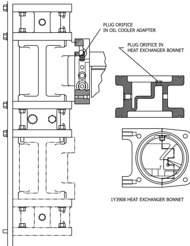
FIG. A6.9 Engine Oil Heating Hardware
