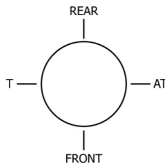
FIG. A13.2 Liner Thrust and Anti-Thrust Locations
