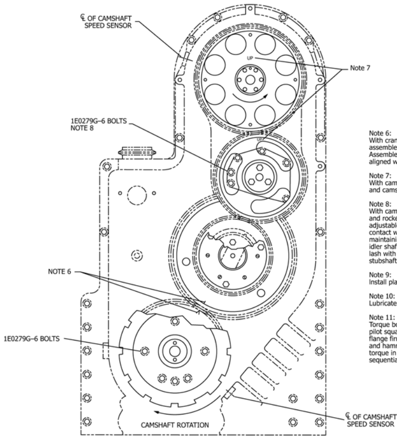
FIG. A10.6 1Y3700 Engine Timing
