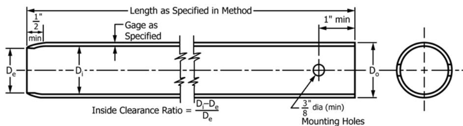
FIG. 2 Thin-Walled Tube Sampler, Practice D1587
