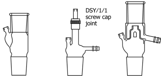
FIG. 3 Basic Head
