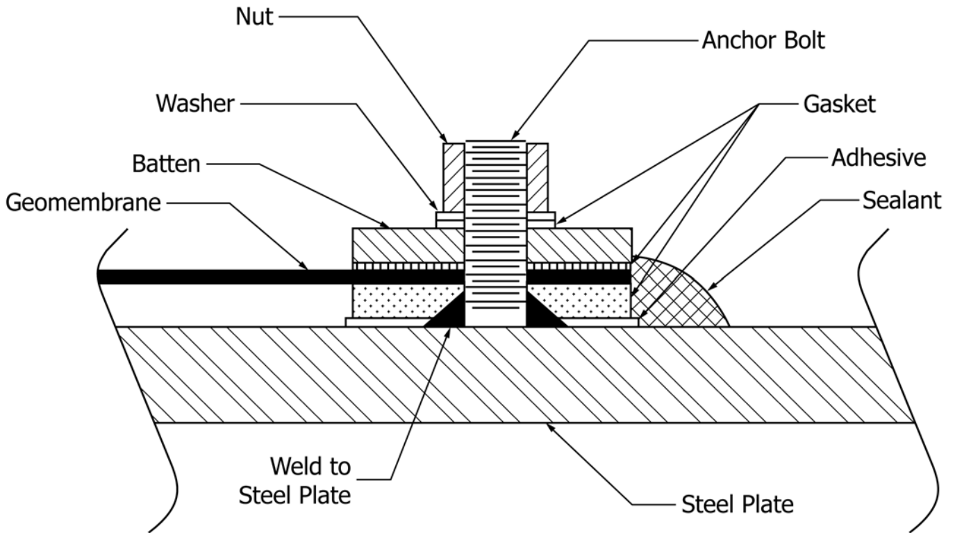
FIG. 11 Batten Attachment to Steel Plate
