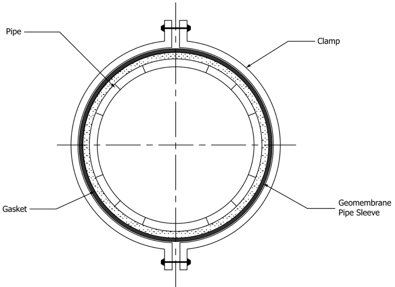
FIG. 2 Clamp Detail
