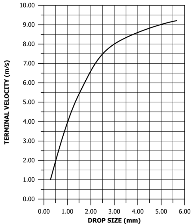
FIG. 7 Terminal Velocity of Distilled Water Droplets in Still Air.
