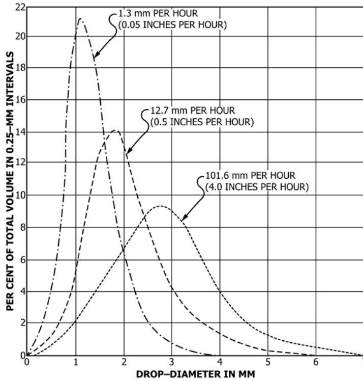
FIG. 5 Example Raindrop Size Distribution
