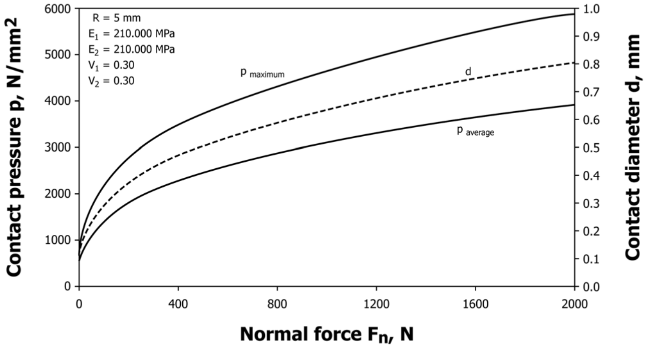
FIG. 6 Evaluation of Hertzian Contact Diameter and Contact Pressure over Test Load
