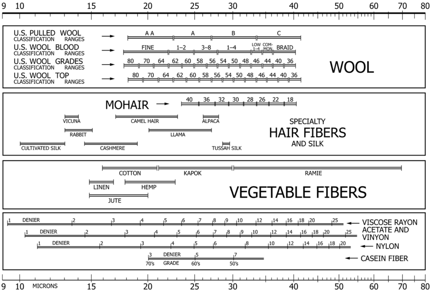
FIG. 1 Comparative Scale for Fineness of Various Textile Fibers
