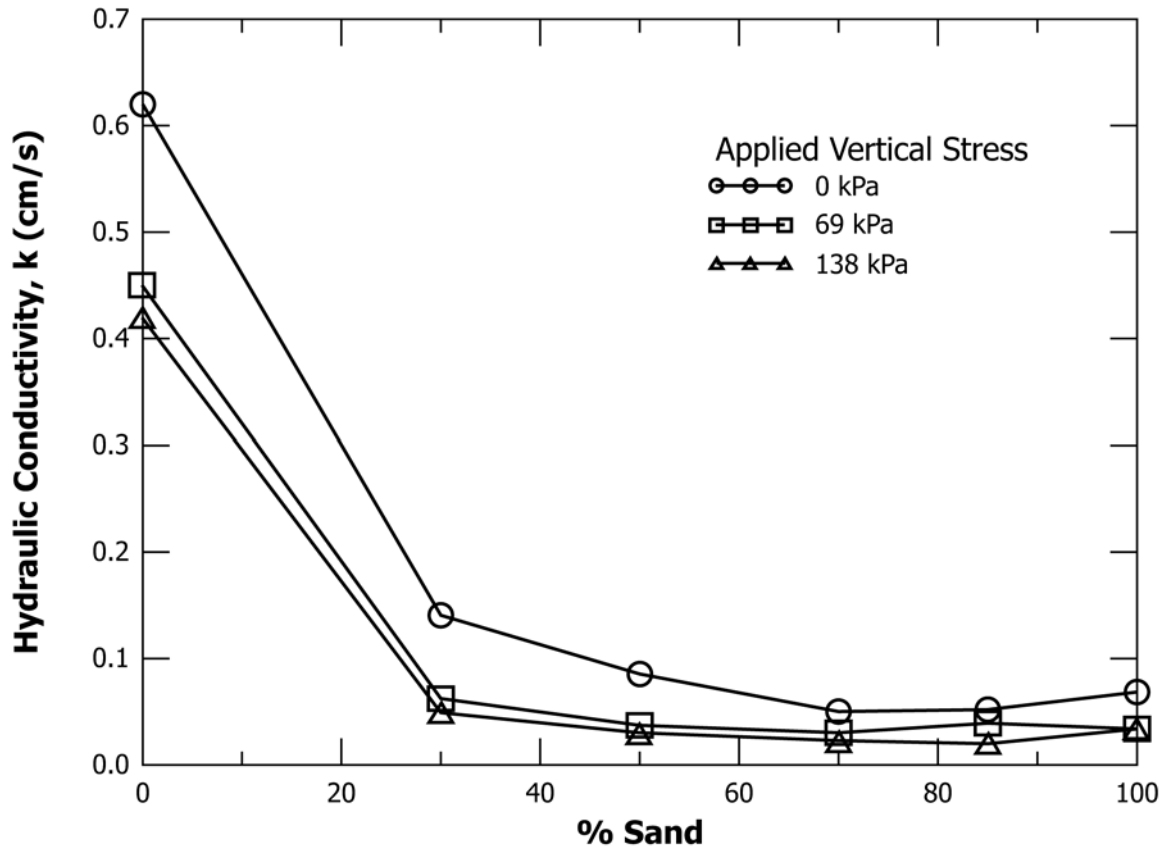
FIG. X1.4 Hydraulic Conductivities of Mixtures of TDA and Clean Sand (4)
