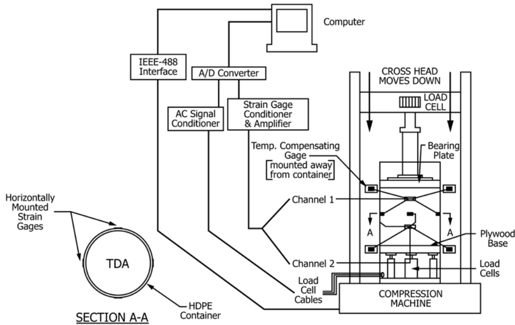
FIG. 1 Compressibility Apparatus for TDA Designed to Measure Lateral Stress and the Portion of the Vertical Load Transferred by Friction from TDA to Container (9)
