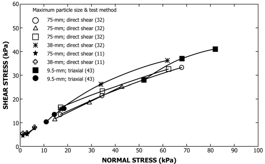
FIG. X1.3 Comparison of Failure Envelopes of TDA at Low Stress Levels
