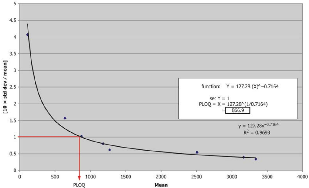
FIG. 1 Fitted Function and Solution for PLOQ Data from Table 1
