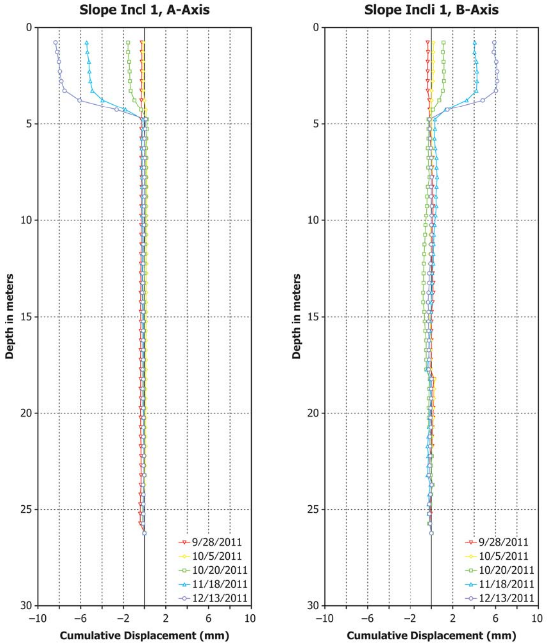
FIG. 4 Displacement Versus Depth and Time
