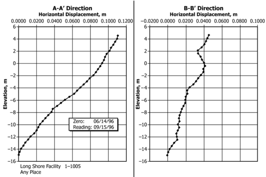
FIG. 3 Plot of Reduced Inclinometer Data
