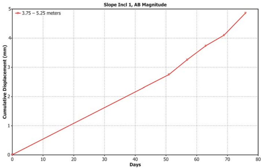
FIG. 5 Displacement Versus Time at Specific Depth Interval
