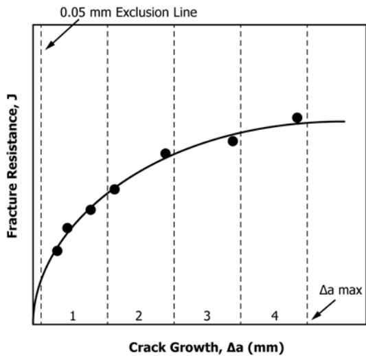
FIG. 7 Data Spacing Requirement
