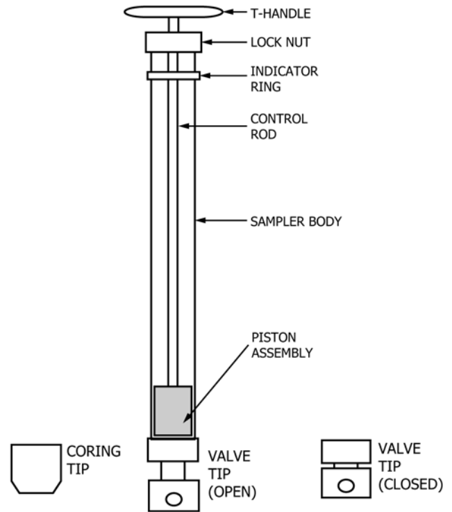
FIG. 14 Syringe Sampler
