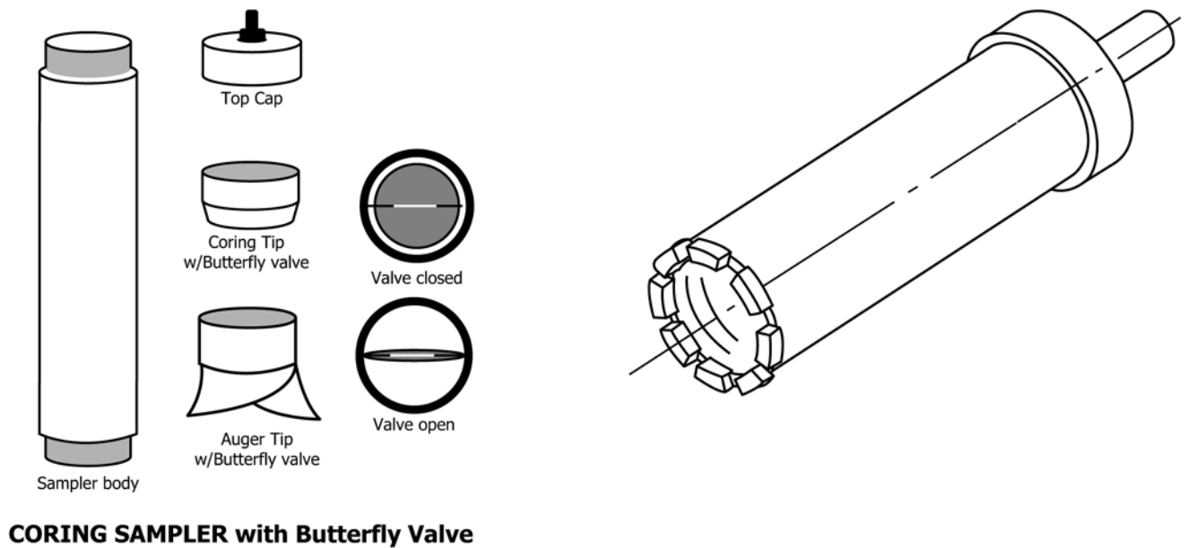
FIG. 7 Coring Devices
