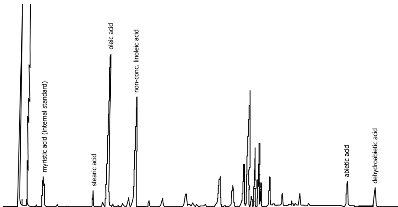
FIG. 1 Typical Chromatogram of Distilled Tall Oil
