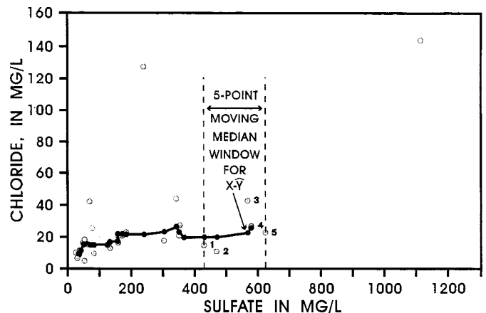
NOTE 1—Adapted from Ref (1). Analyses from Ref (65), see Table 4. FIG. 14 Scatterplot Smoothing by Moving Median
