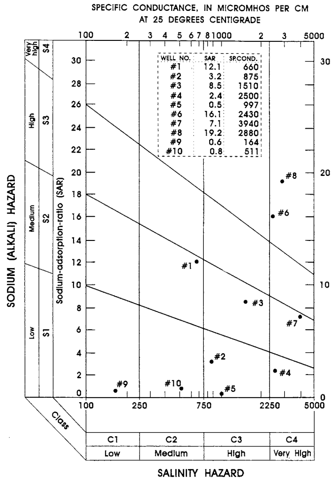
NOTE 1—Adapted from Ref (3). Analyses from Ref (3). FIG. 21 Irrigation Classification Diagram
