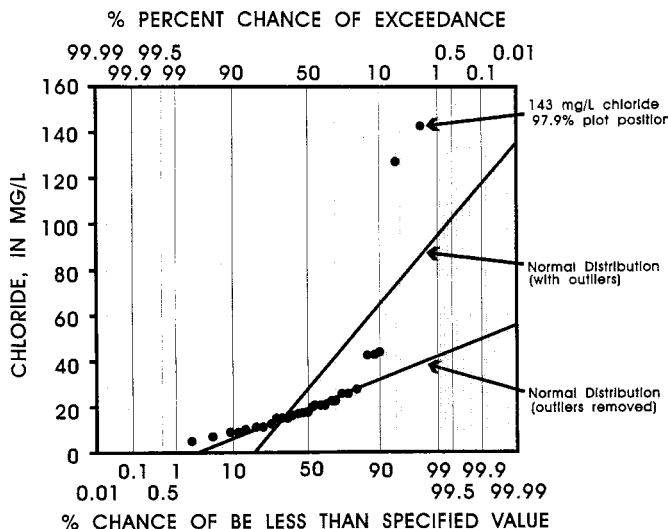
NOTE 1—Analyses from Ref (65), see Table 3. FIG. 11 Probability Plot Using Percent
