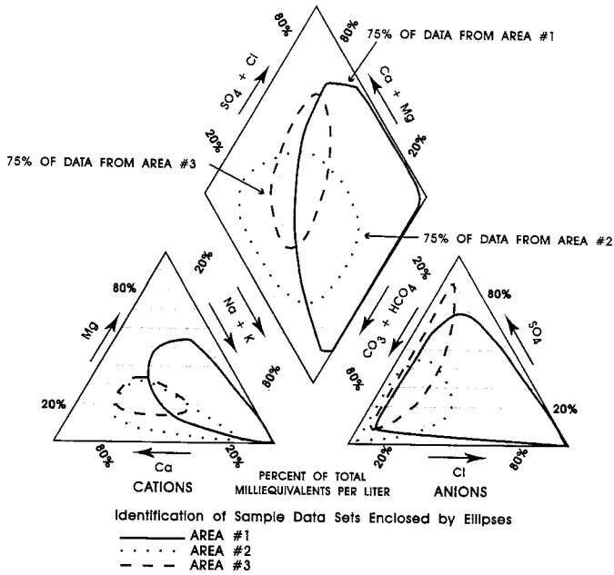
NOTE 1—Adapted from Ref (12). FIG. 22 Piper Diagram With Polar Smoothing
