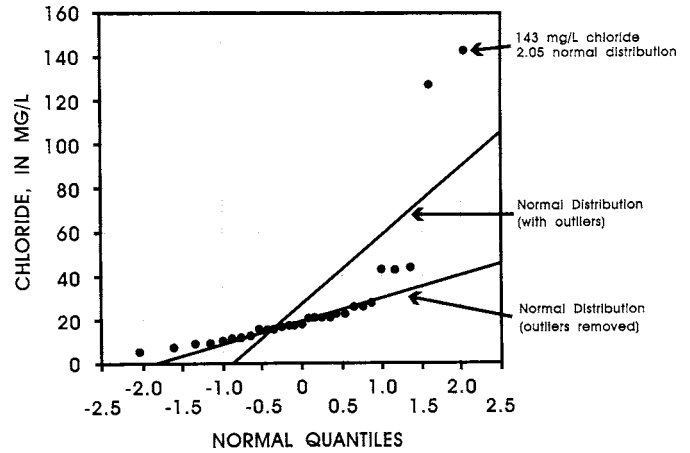
NOTE 1—Analyses from Ref (65), see Table 3. FIG. 12 Probability Plot Using Quantiles
