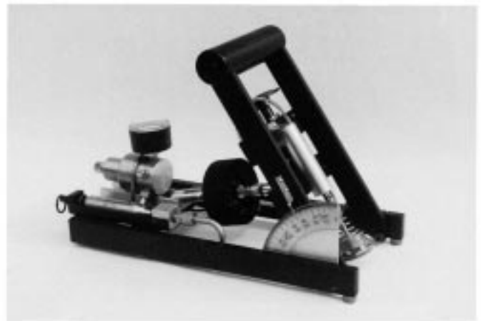
FIG. 1 Variable Incidence Tester
