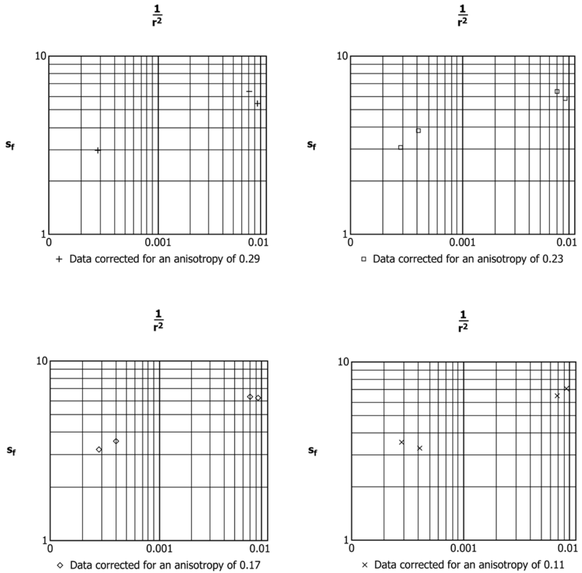
FIG. 4 Graphs of Corrected Drawdown in Feet Versus Reciprocal of Distance Squared in \text{ft}^2 ( \text{m}^2 ) for Anisotropy Ratios of 0.29, 0.23, 0.17, and 0.11, a T of 35.42 \text{ ft}^2 ( 3.29 \text{ m}^2 )/day, and an S of 0.00055
