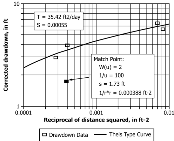
FIG. 3 Analysis of Drawdown Data Corrected for Partial Penetration Assuming an Anisotropy of 0.20, Estimated T of 53.48 \text{ft}^2 ( 4.97 \text{ m}^2 )/day, and S of 0.0005 Yields a Revised T of 35.42 \text{ft}^2 ( 3.29 \text{ m}^2 )/day and S of 0.00055
