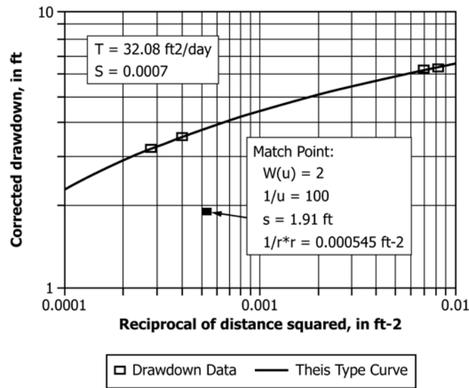
FIG. 7 Analysis of Drawdown Data Corrected for Partial Penetration Assuming an Anisotropy of 0.18, Estimated T of 32.77 ft 2 (3.04 m 2 /day, and S of 0.00065 Yields a Revised T of 32.08 ft 2 (2.98 m 2 /day and S of 0.0007
