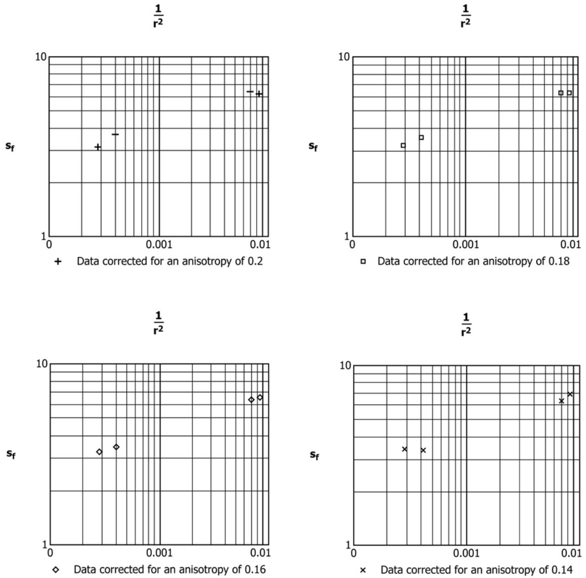
FIG. 6 Graphs of Corrected Drawdown in Feet Versus Reciprocal of Distance Squared in \text{ft}^2 ( \text{m}^2 ) for Anisotropy Ratios of 0.2, 0.18, 0.16, and 0.14, a T of 32.77 \text{ ft}^2 ( 3.04 \text{ m}^2 )/day, and an S of 0.00065
