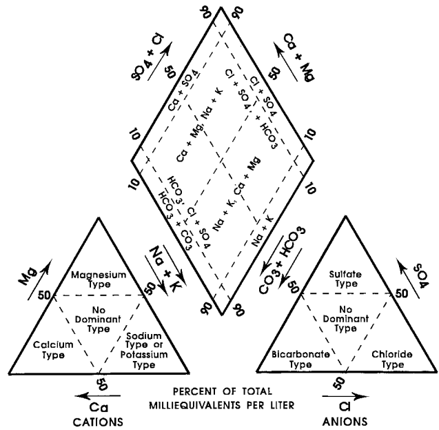
FIG. 16 Piper Diagram Showing Classification of Hydrochemical Facies (Adapted from Ref (47))
