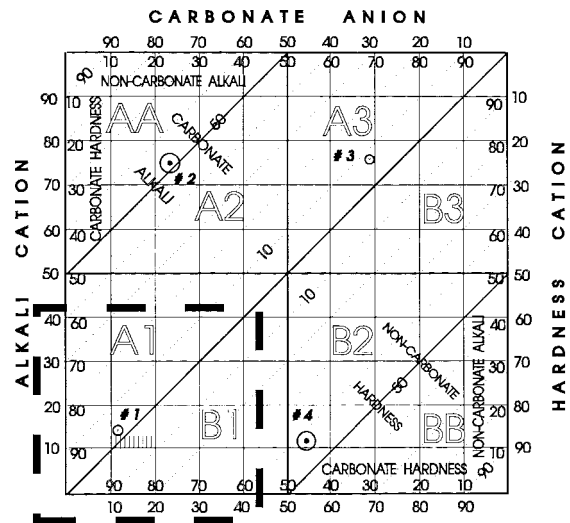
PERCENT OF TOTAL MILLIGRAM EQUIVALENTS PER LITER (See Table 5 for Analyses)
