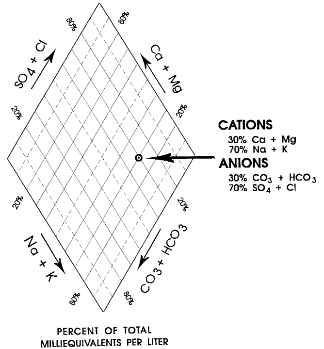
PERCENT OF TOTAL MILLIEQUIVALENTS PER LITER FIG. 10 Example of Diamond Diagram (Adapted from Refs (5) and (6))
