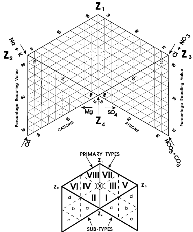
FIG. 1 Geochemical Pattern Diagram (Adapted from Refs (1) and (4))
