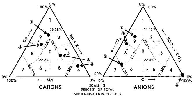
● Plot Position of Analysis from Table 2 Alinement of 50 Percent Unit Line FIG. 8 Carreno Trilinear Classification Diagram (Adapted from Ref (35))
