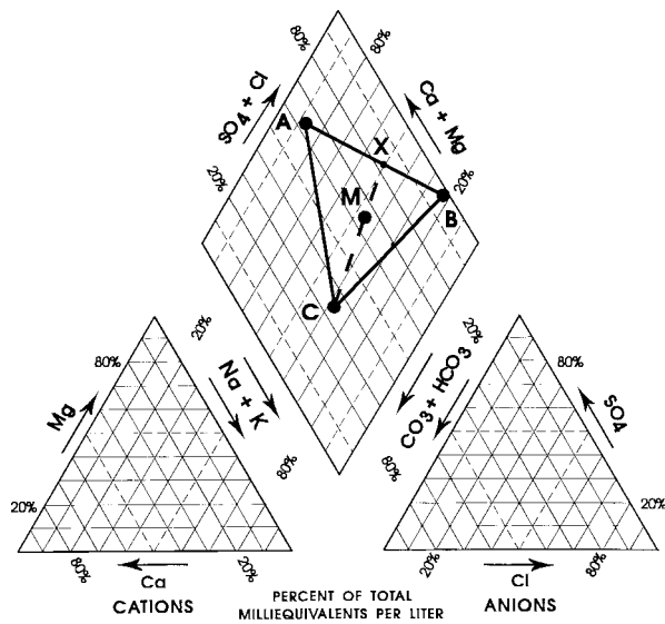
FIG. 14 Example of Piper Diagram Showing Mixture of Two Parent Waters (Adapted from Ref (5))
