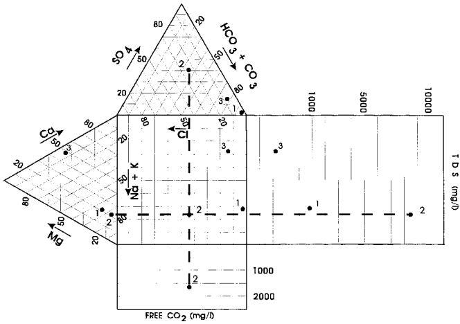
FIG. 19 Example of Durov Water Classification Diagram (Adapted from Ref (43))
