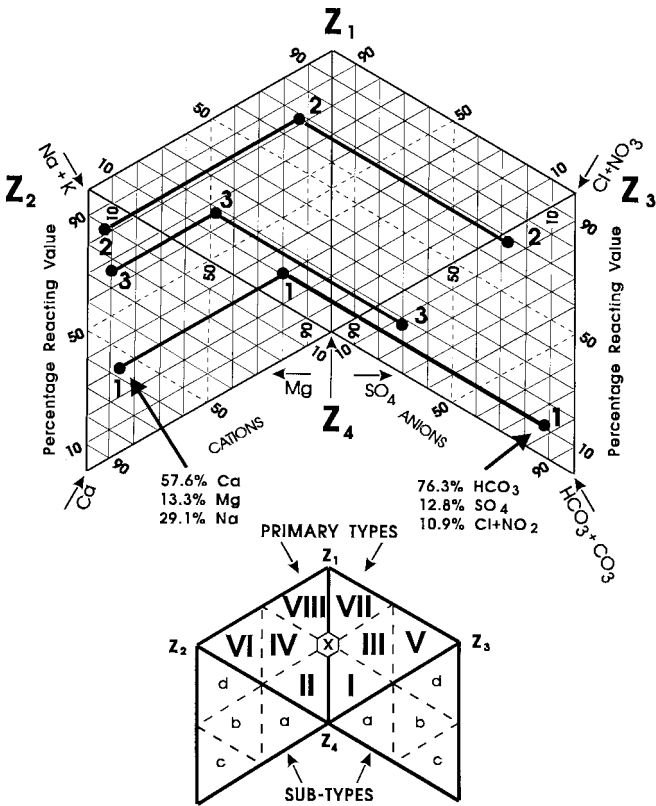
FIG. 12 Example of Hill Geochemical Pattern Diagram (Adapted from Ref (1))
