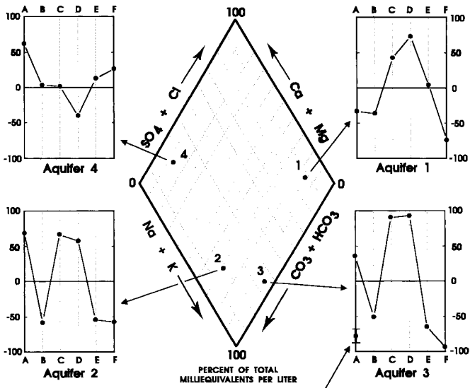
NOTE: Multiple Analyses From A Source Are Shown By The Following Symbol -- I Maximum Minimum FIG. 7 D'Amore, et al Classification Diagram (see Table 4 for Plotted Parameters)
