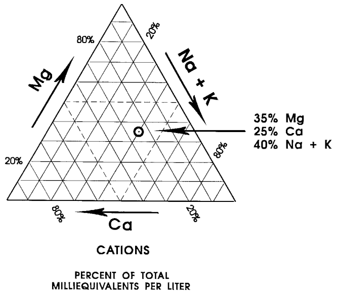
PERCENT OF TOTAL MILLIEQUIVALENTS PER LITER FIG. 9 Example of Trilinear Plot (Adapted from Refs (5) and (6))
