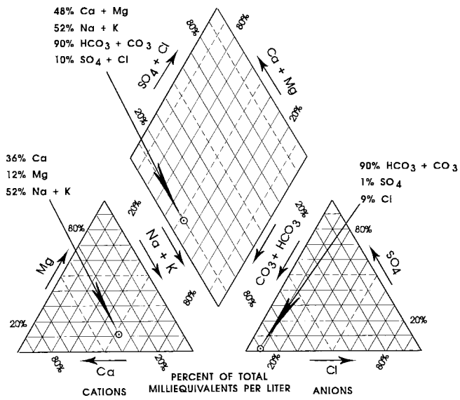
FIG. 11 Example of Water Analysis Diagram (Adapted from Refs (5) and (6))
