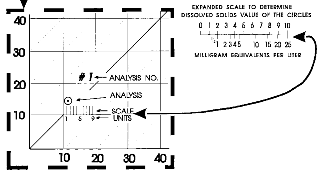
FIG. 13 Example of Water Classification Diagram (Adapted from Ref (4))
