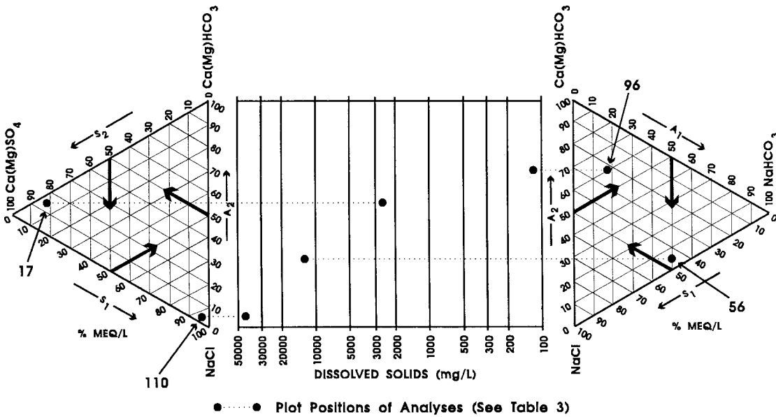
FIG. 6 Filatov and Gazda Trilinear Diagrams: ( a ) Filatov Graphical Representation of Water Chemistry (Adapted from Ref (31)), and ( b ) Gazda Classification Diagram of Chemistry of Mineral Water (Adapted from Ref (32))
