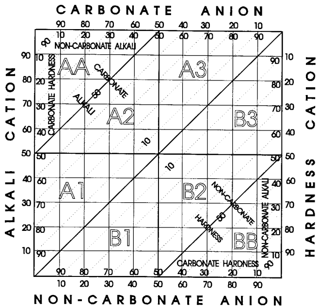
FIG. 2 Water Classification Diagram (Adapted from Ref (4))
