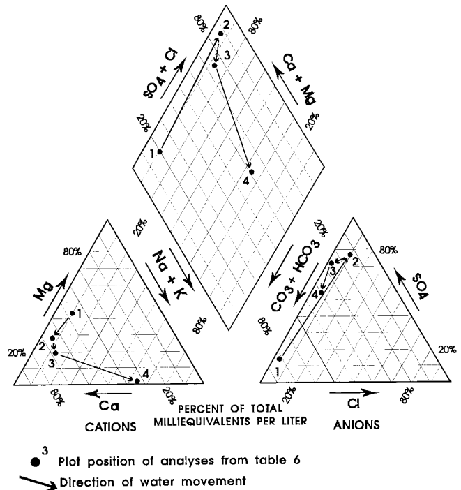
FIG. 17 Example of Piper Diagram Showing Chemical Changes from Recharge (1) to Discharge Area (4) (Adapted from Ref (48))
