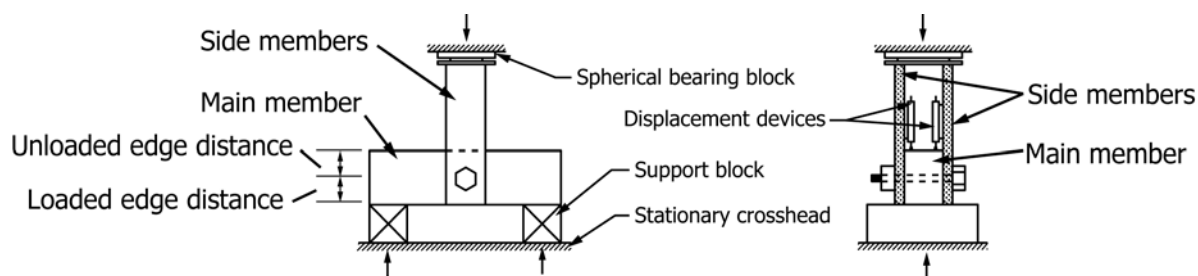
FIG. 3 Assembly for Testing Single-Bolt Connections Perpendicular to Grain in Compression
