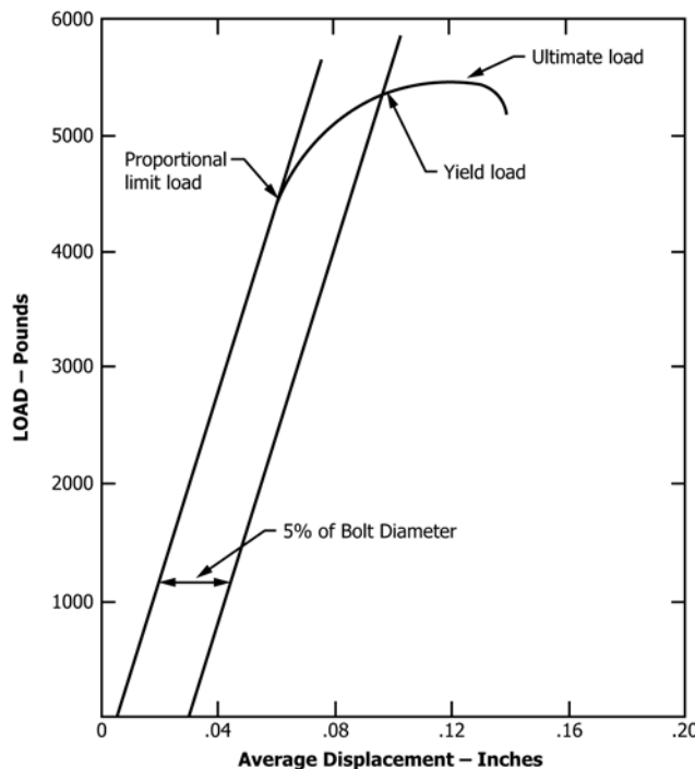
FIG. 4 Definition of Loads to Be Obtained from the Load-Displacement Curve
