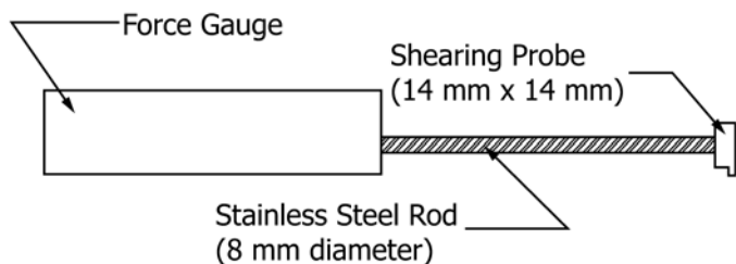
FIG. 1 Probe Design for the Detachment of Barnacles
