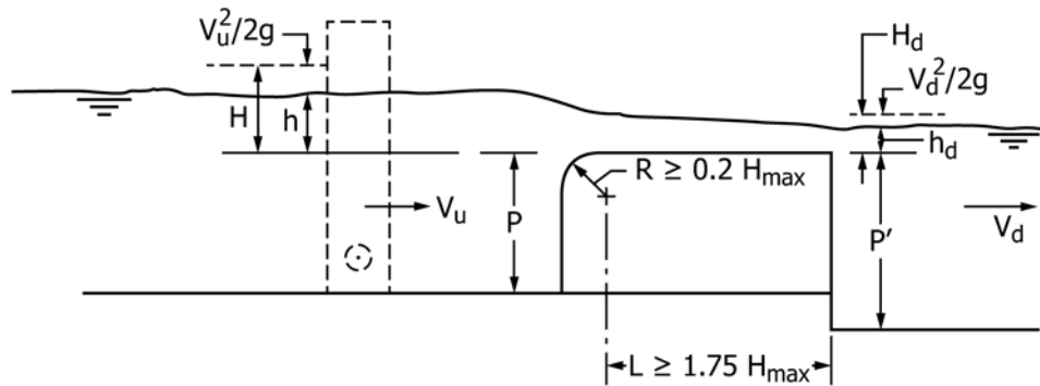
FIG. 3 Rounded Broad-Crested Weir
