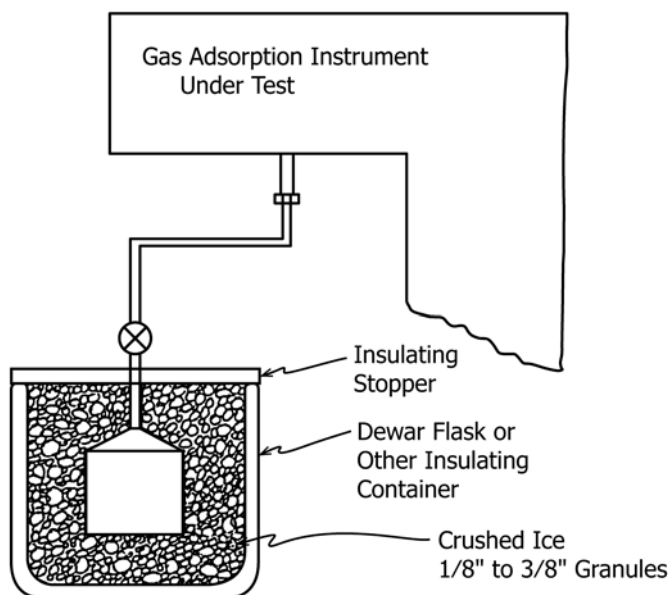
FIG. 2 Volumetric Apparatus Installed and Readied for Gas Adsorption Instrument Calibration Verification
