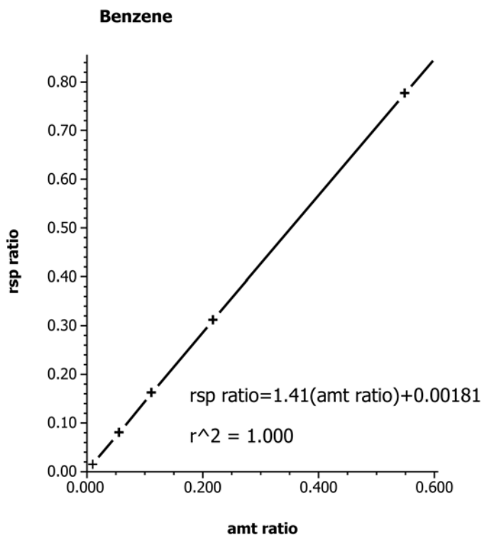
FIG. 3 Typical Benzene Calibration Curve
