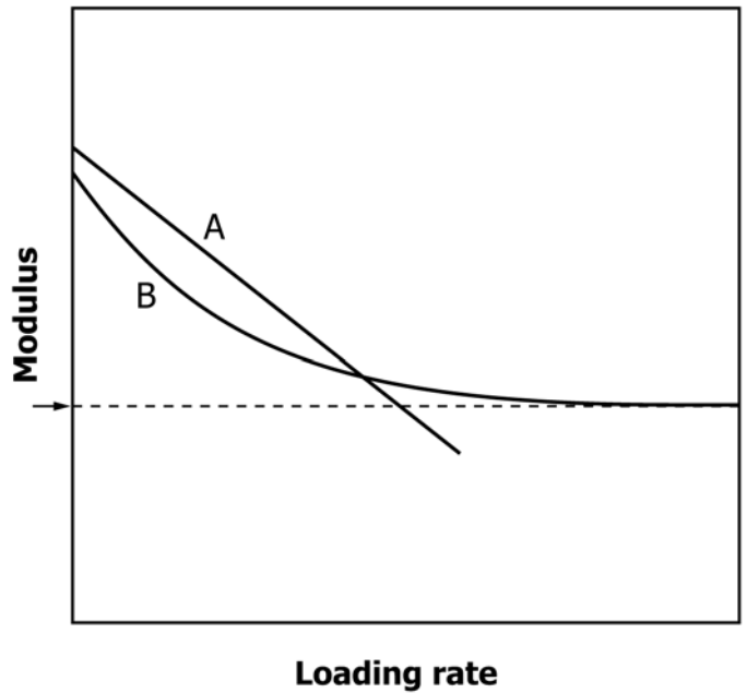
NOTE 1—With decreasing rate of loading until the joint either fails or approaches an asymptotic value for the applied stress level and the environmental conditions.
