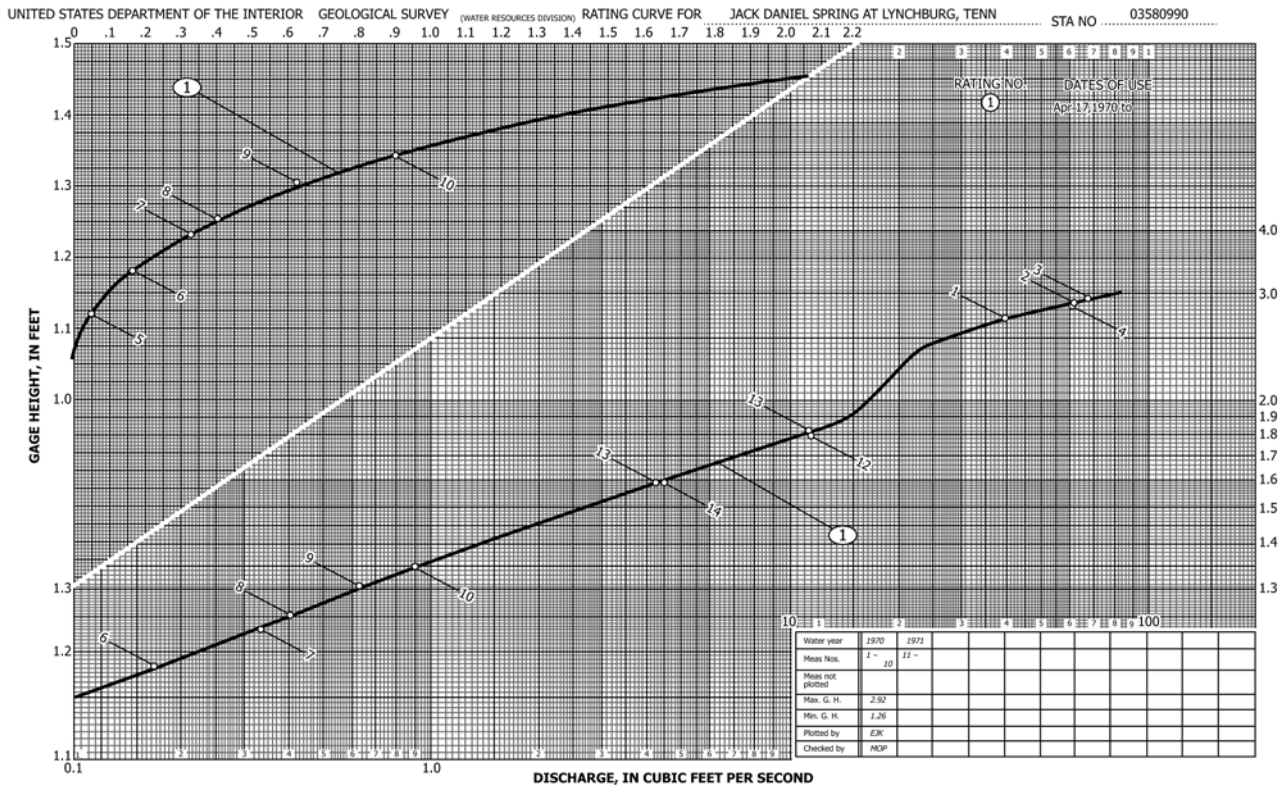
FIG. 1 Typical Rating-Curve Sheet
