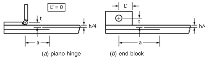
FIG. A1.1 Methods for Introducing Opening Load to DCB Specimens
