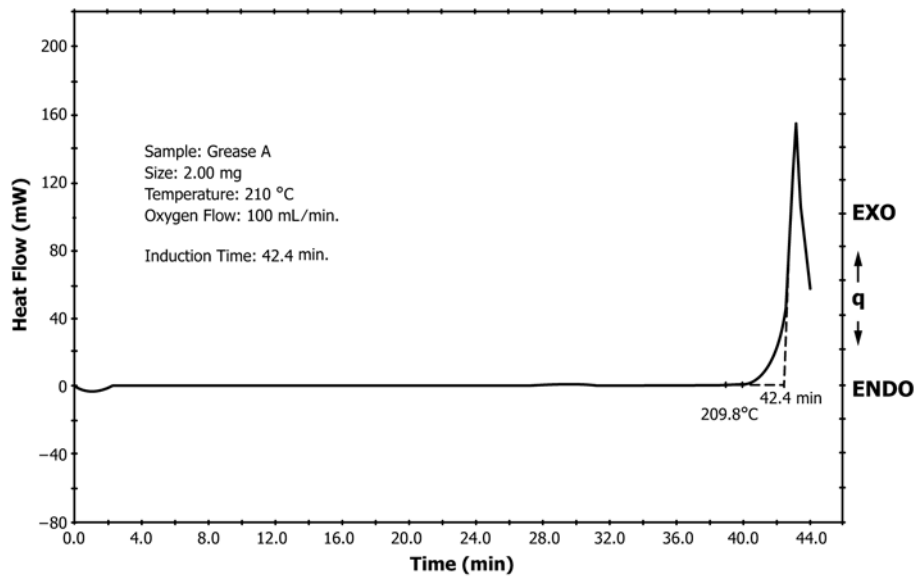
FIG. 4 Typical PDSC Thermal Curve
