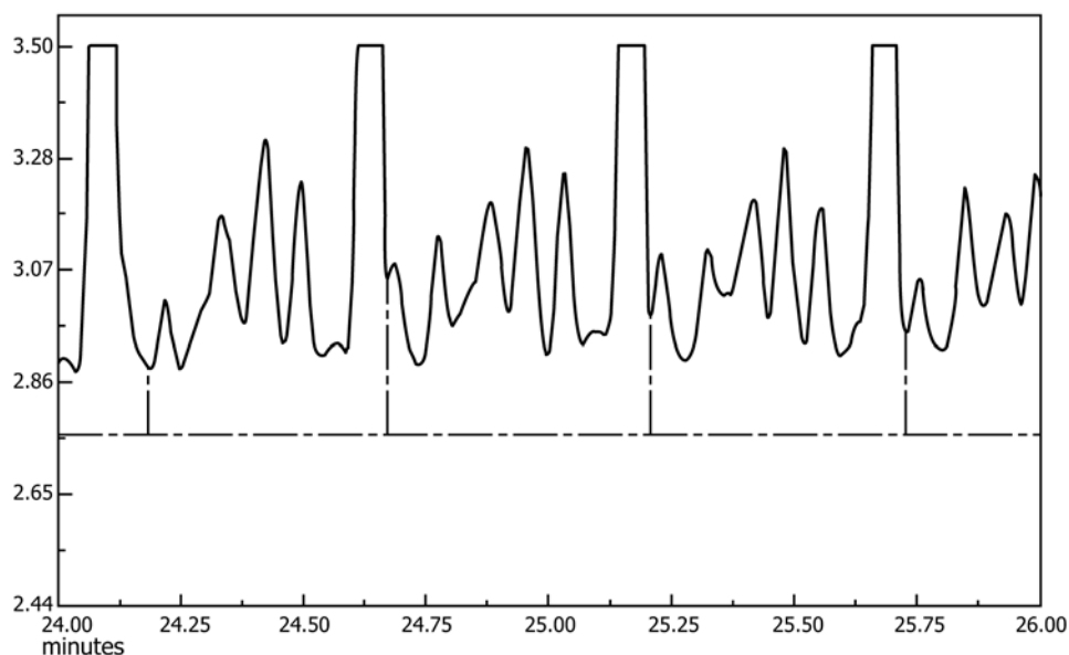
FIG. 3 Carbon Number Summation (Vertical Drop to Horizontal Baseline)
