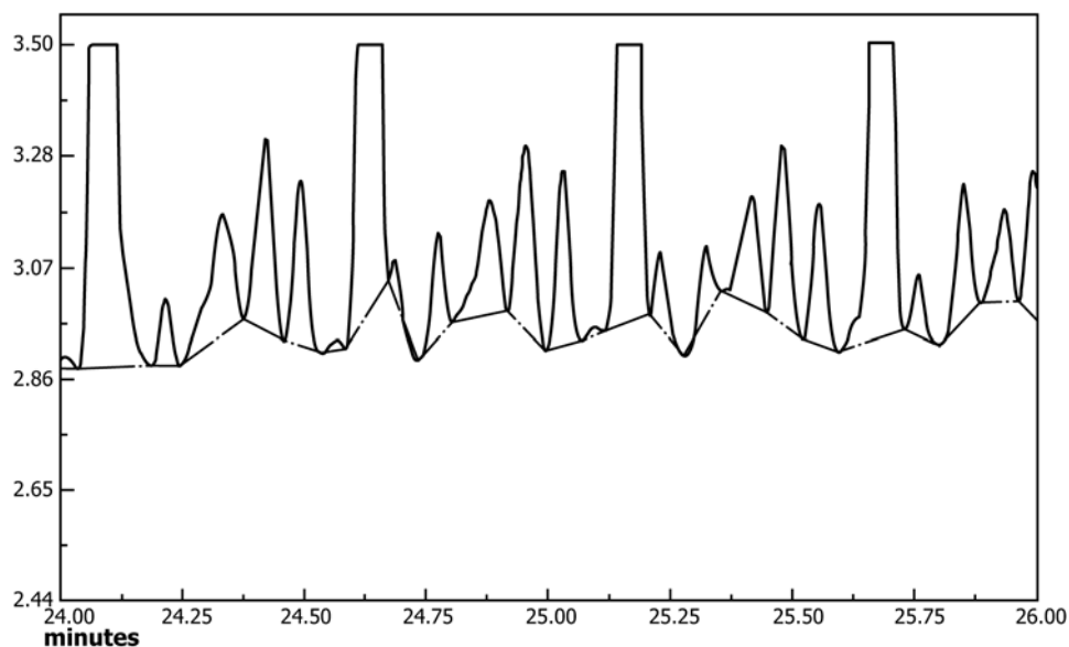
FIG. 2 Valley to Valley Integration for Area of Normal Paraffin
