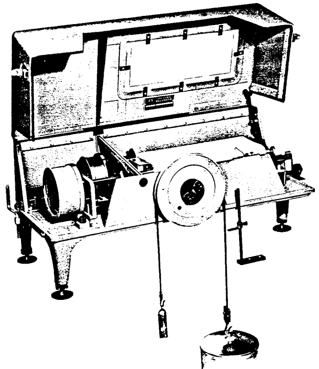
FIG. 8 Graphic Recorder
