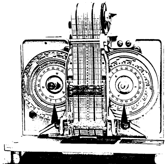
FIG. 9 Digital Recorder
