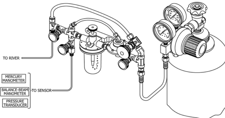
FIG. 7 Gas-Purge System
