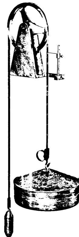
FIG. 4 Float-Type Gauge
