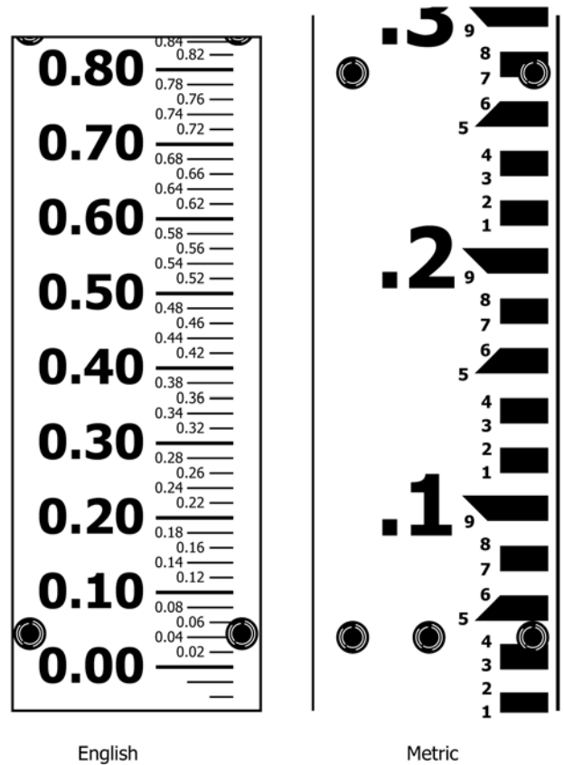
FIG. 1 Staff Gauges
