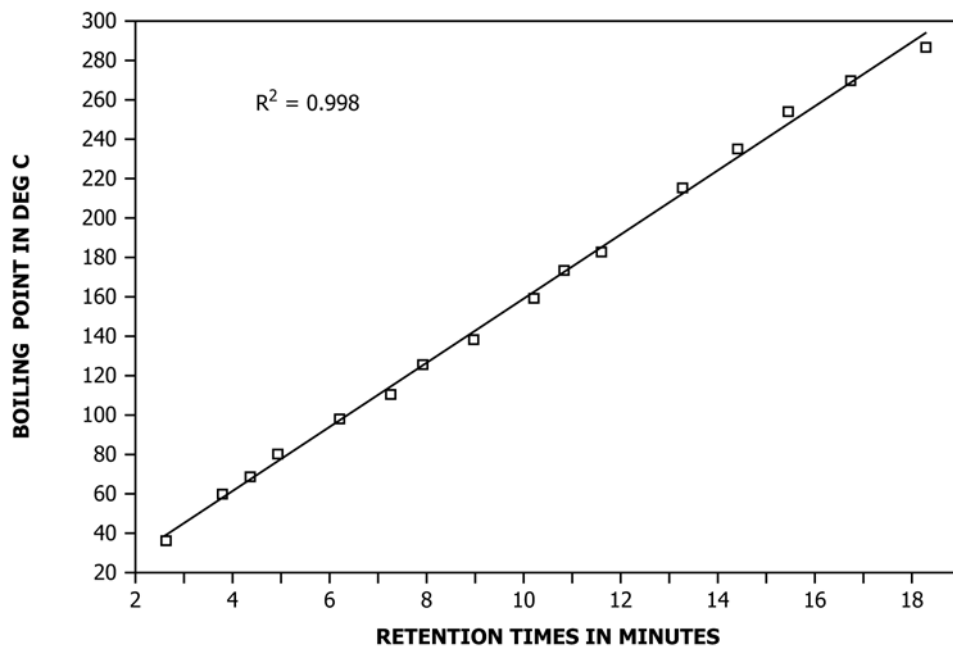
FIG. 3 Calibration Curve
