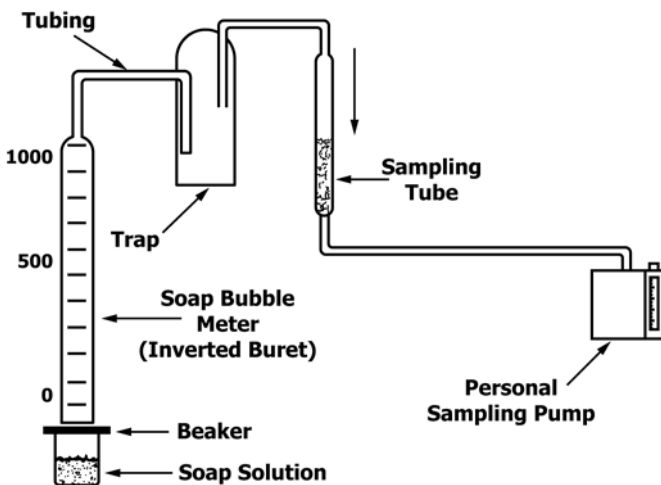
FIG. 2 Calibration Setup for Personal Sampling Pump with Sampling Tube
