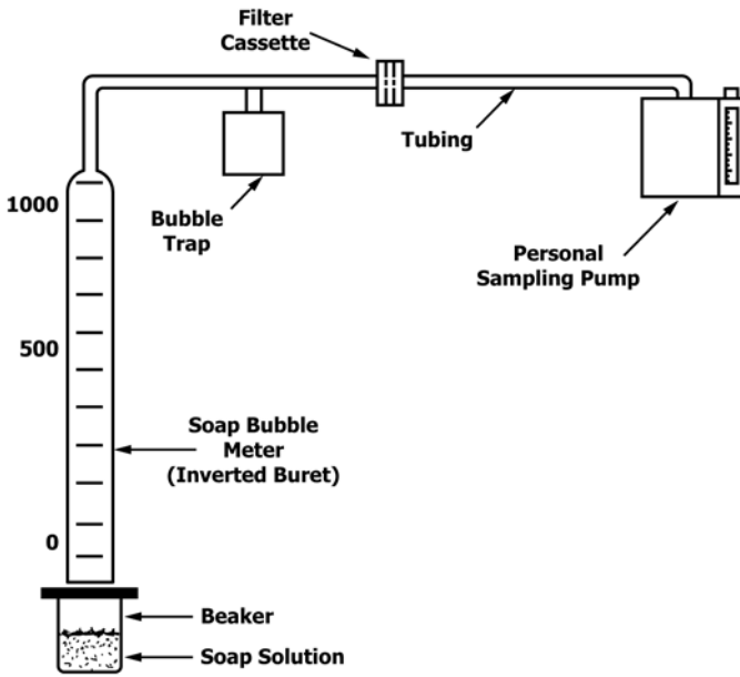
FIG. 1 Calibration Setup for Personal Sampling Pump with Filter Cassette
