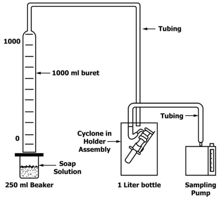
NOTE 1—Other cyclones may require different setups. FIG. 3 Calibration Setup for Personal Sampling Pump with a 10-mm Nylon Cyclone Respirable Dust Sampler Using a Bubble Meter
