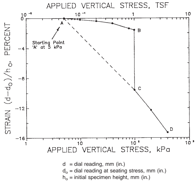
NOTE 1— (d - d_0)/h_0 is multiplied by 100 to obtain percent. FIG. 1 Example Compression Curve of the Collapse Potential Test
