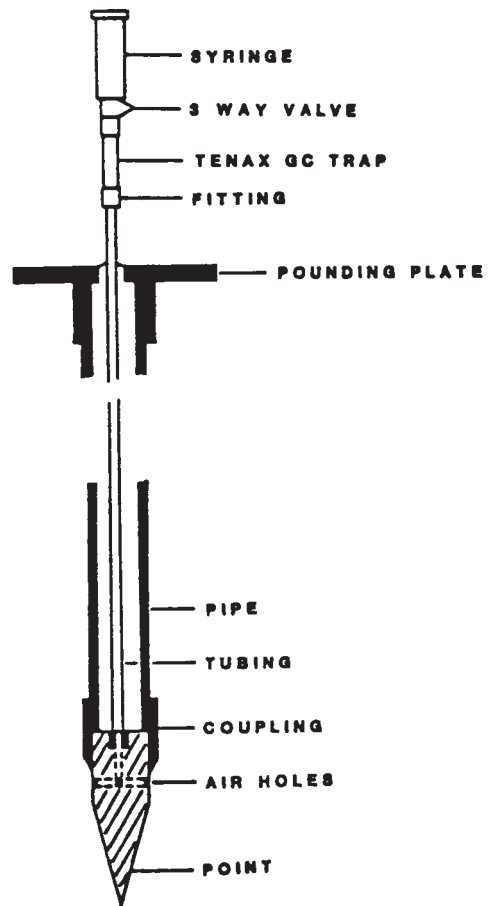
FIG. X1.4 Example of Sorbed Contaminant-Active System
