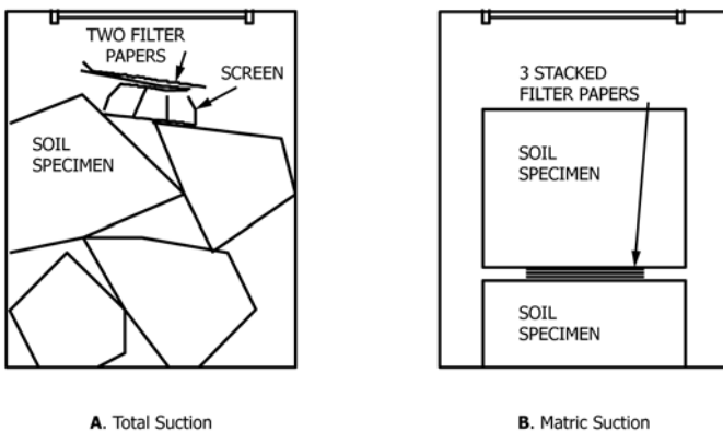
FIG. 2 Setup for Equilibrating Suction in Large Container
