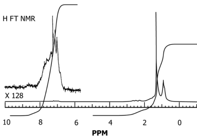
FIG. 1 80 MHz 1 H NMR Spectrum of a Gas Oil
