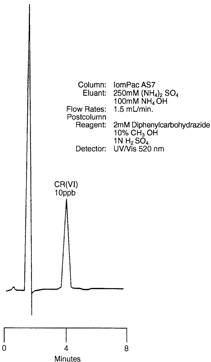
FIG. 3 Ion Chromatographic Determination of Hexavalent Chromium
