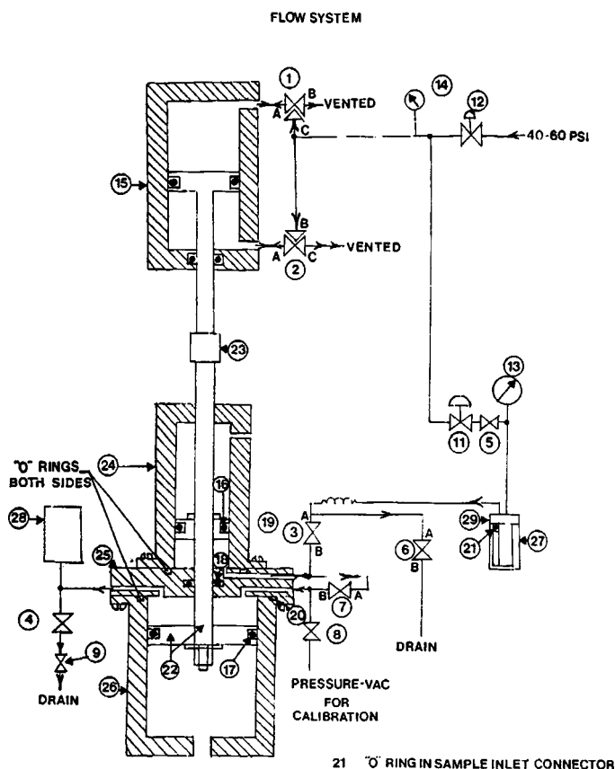
FIG. A1.1 Flow System for Automatic Vapor Pressure Instrument
