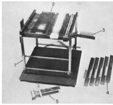
(Front View) 1—Frame. 2—Faller bars. 3—Side comb. 4—Retaining bars. 5—Drawing clamp.
