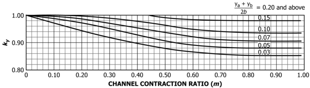
B. Adjustment factor variation with \frac{y_a + y_b}{2b} ratio
