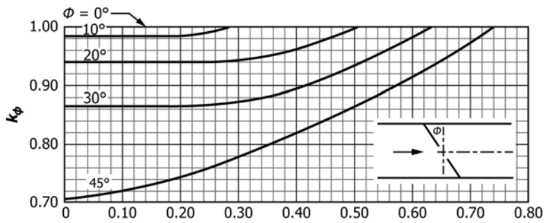
B. Adjustment factor variation with angularity
