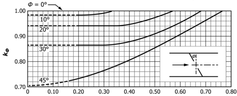
B. Adjustment factor variation with angularity
