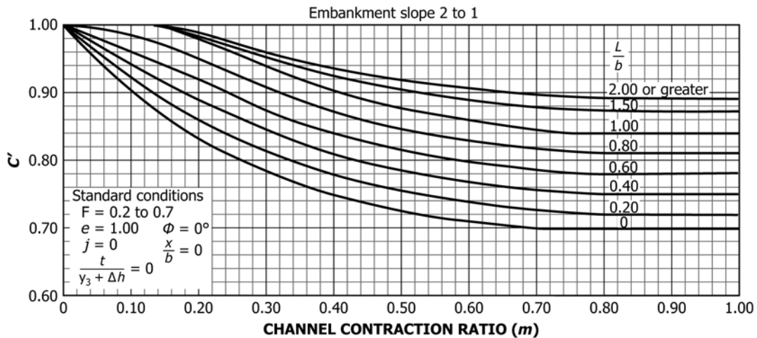
A. Curves for base coefficient of discharge
