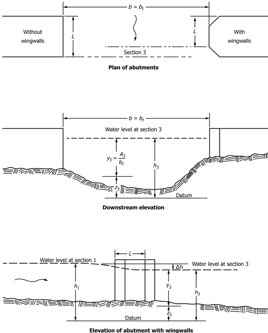
FIG. 3 Definition Sketch of Type 1 Opening, Vertical Embankments and Vertical Abutments With or Without Wingwalls
