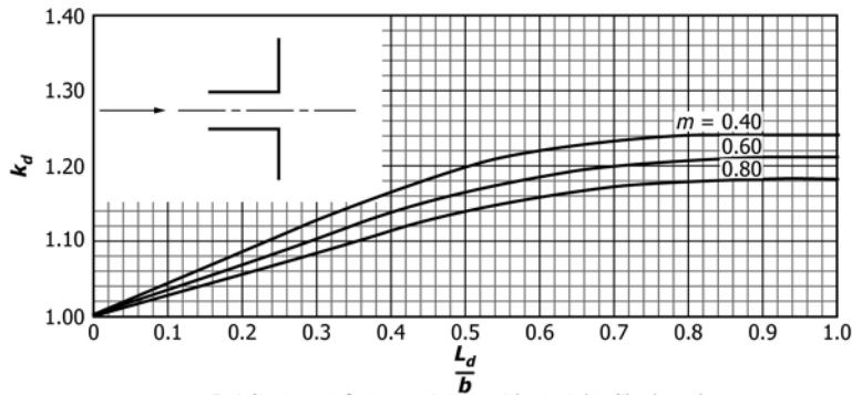
C. Adjustment factor variation with straight dike length
