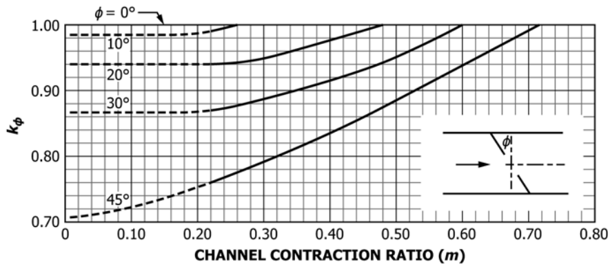
C. Adjustment factor variation with angularity
