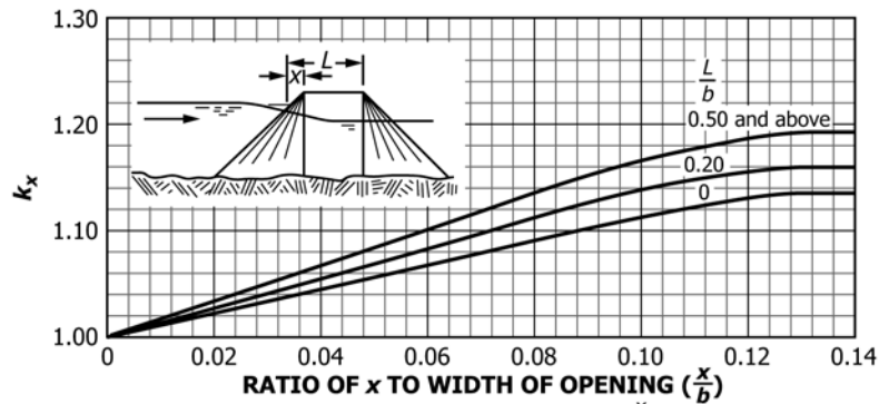
C. Adjustment factor variation with \frac{x}{b} ratio
