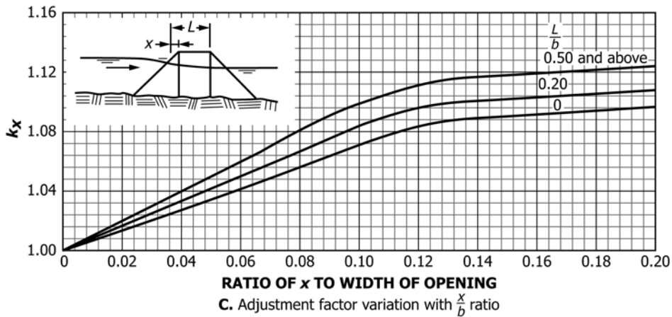
FIG. 12 Coefficients for Type 3 Opening, Embankment and Abutment Slope 1½ to 1
