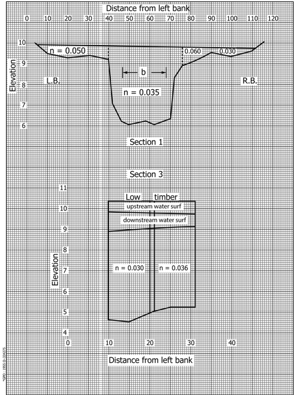
FIG. 27 Sample Contracted-Opening Computation, Bridge Geometry
