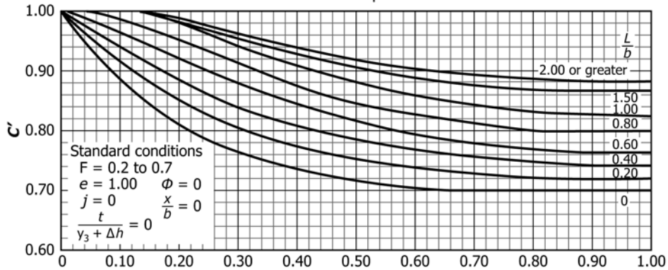
A. Curves for base coefficient of discharge
