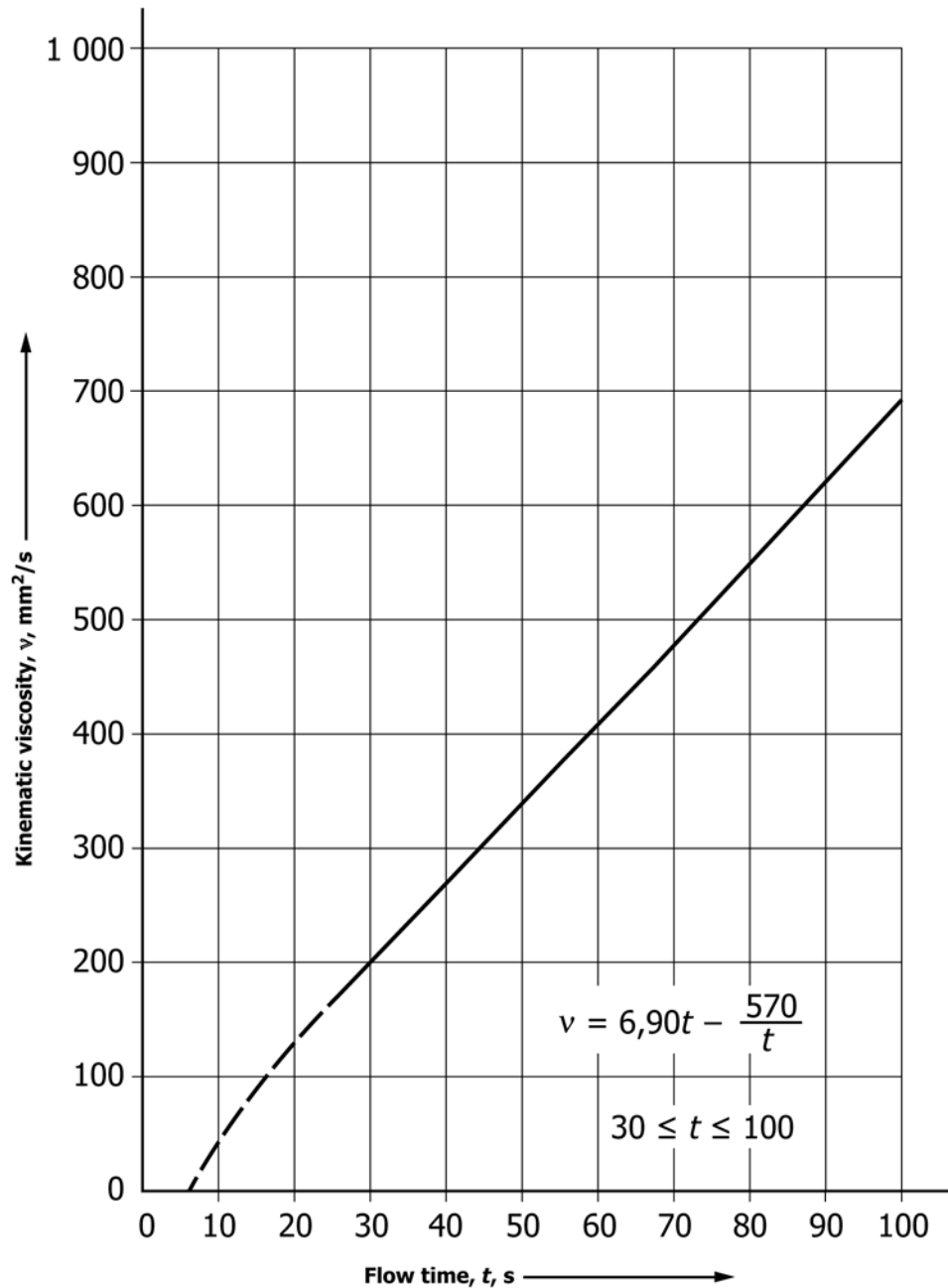
FIG. 5 Calibration Curve for 6-mm Cup
