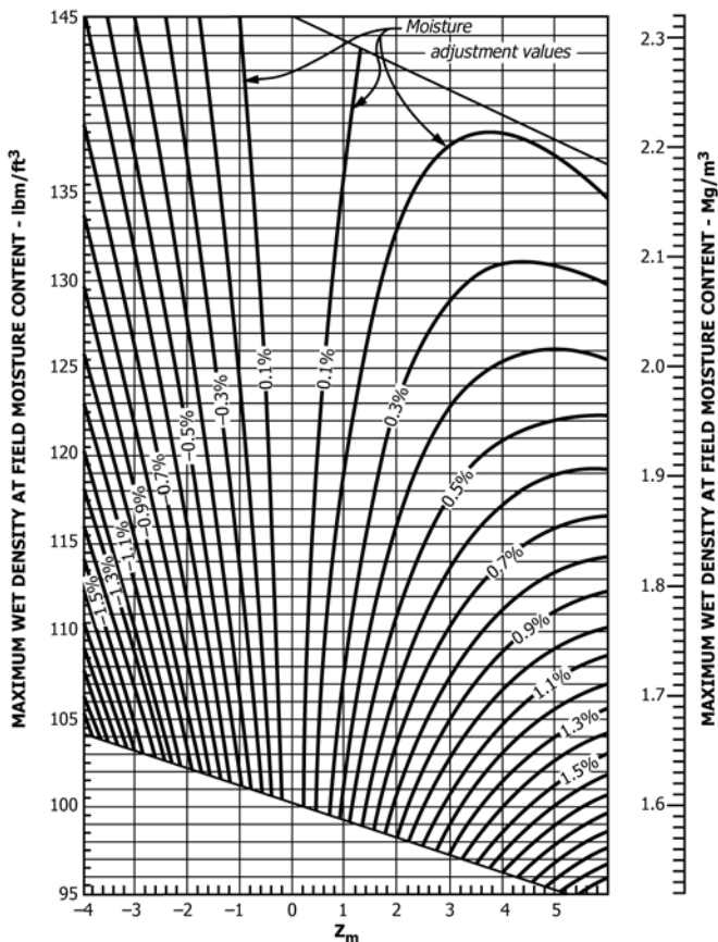
FIG. 2 Water Content Adjustment Values
