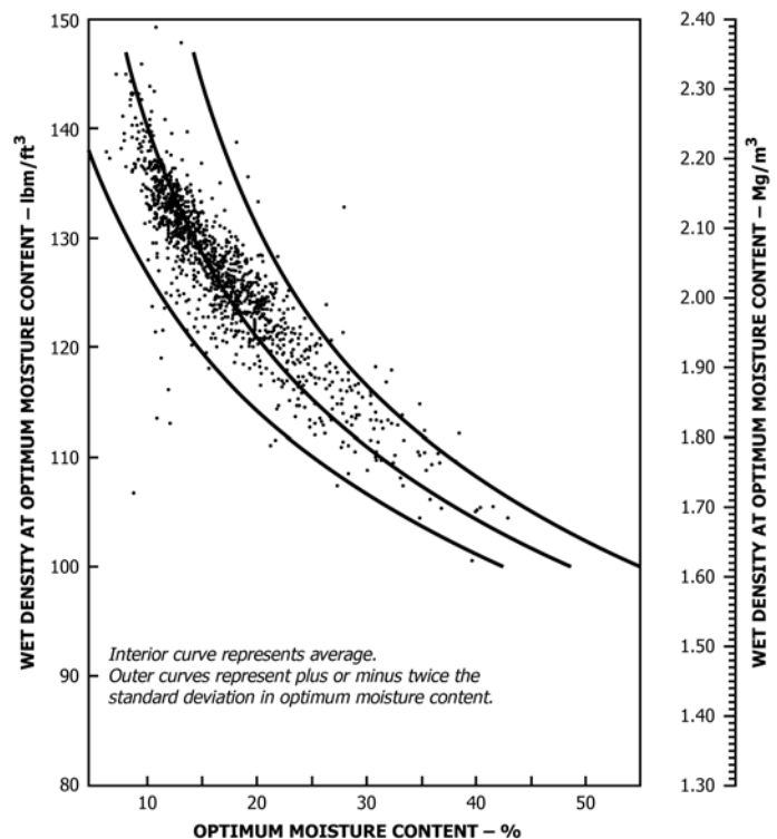
FIG. X2.1 Wet Density Versus Optimum Water Content
