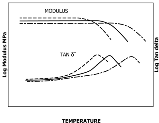
FIG. 1 Dynamic Mechanical Properties in Tension (at Different Frequencies)
