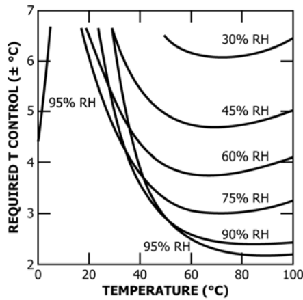
FIG. X1.3 Temperature Control Required to Maintain EMC of Solid and Composite Wood Products within ±0.25 % MC (Ref (4))
