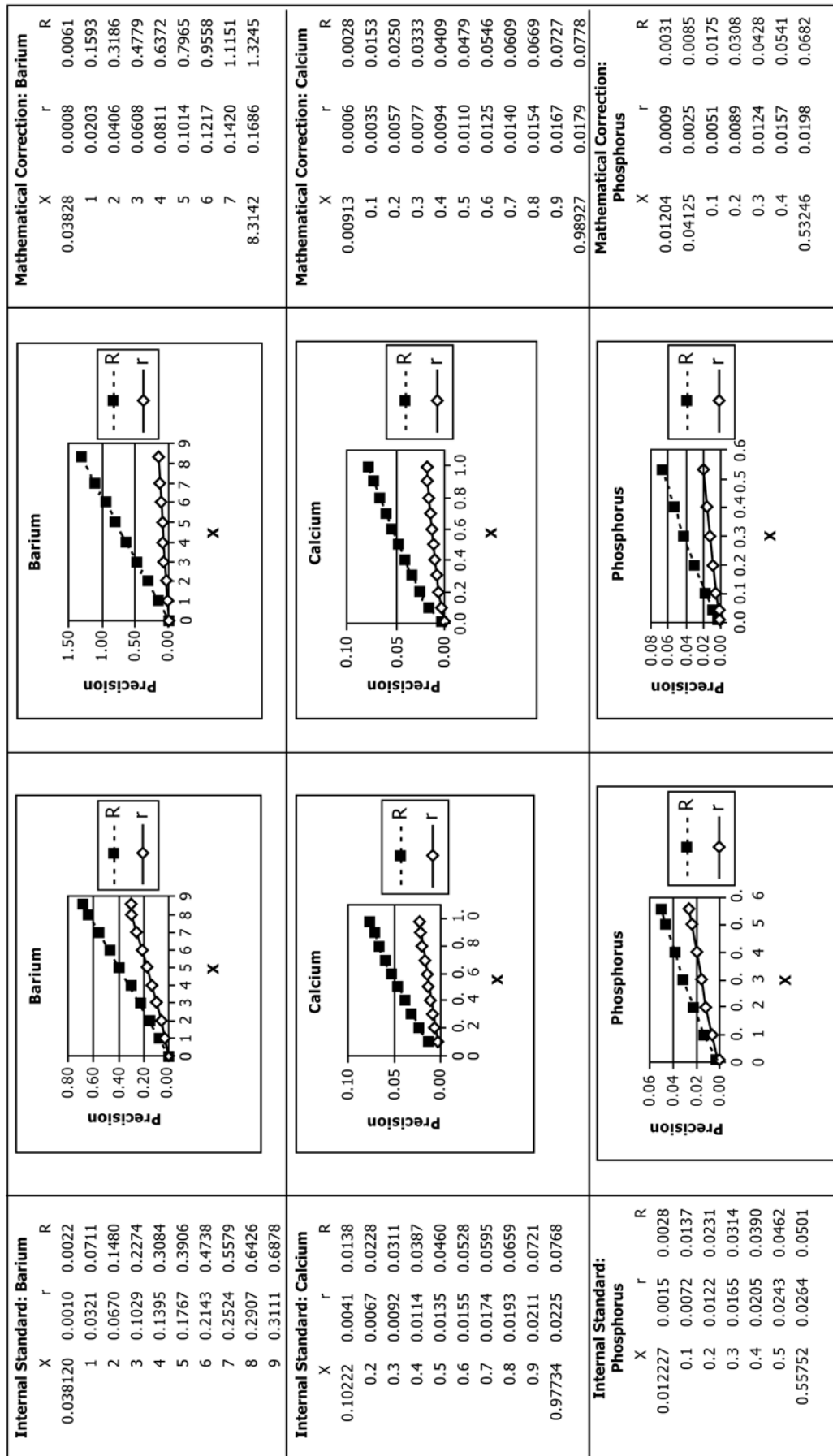
FIG. 1 Repeatability, r, and Reproducibility, R, at Selected Values
