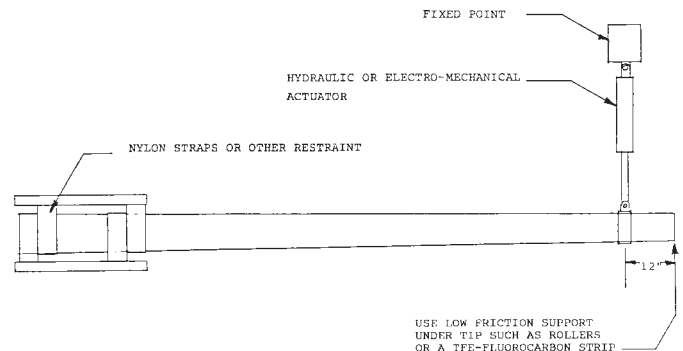
FIG. 9 Plan View of Cyclic Test Apparatus
