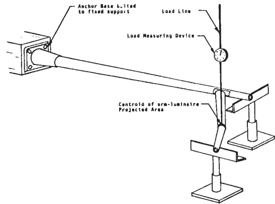
FIG. 7 Anchor-Base Torsional Test Setup
