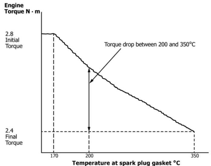
FIG. 2 Torque/Temperature Trace
