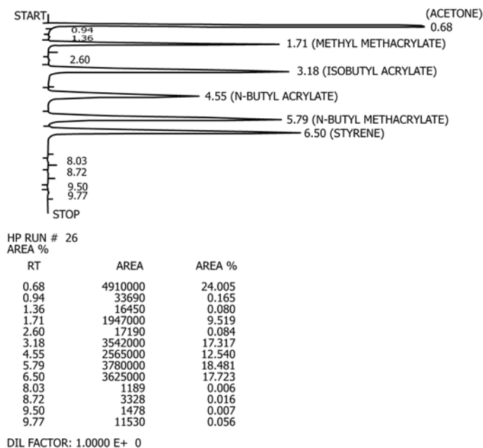
FIG. 1 Typical Chromatogram
