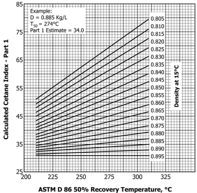
FIG. 1 Calculated Cetane Index
