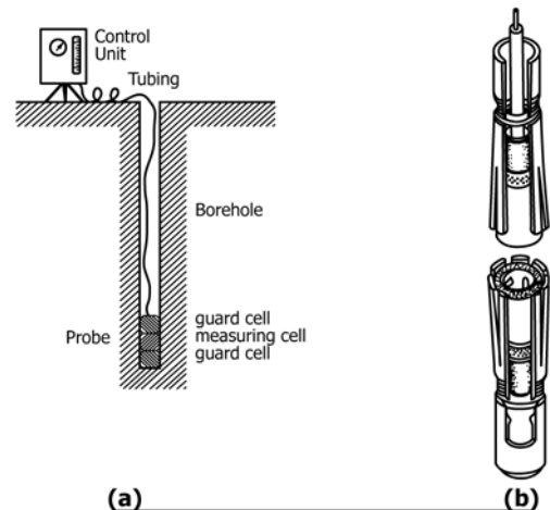
FIG. 1 a) Basic Principles of the Triple Cell Design Pressuremeter (Baguelin, Jézéquel and Shields, 1978, 3 b) Slotted Tube with Probe
