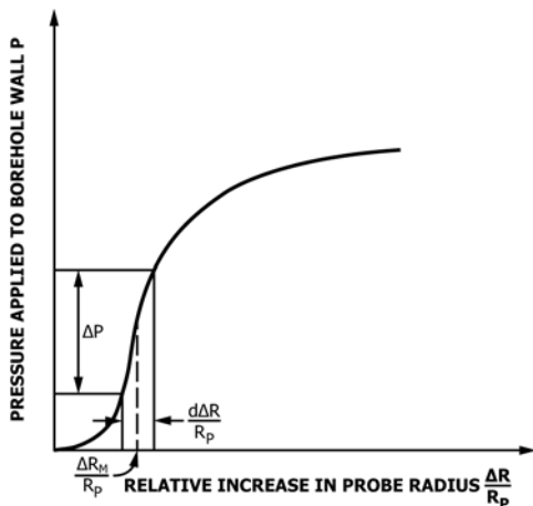
FIG. 9 Pressure Versus Relative Increase in Radius
