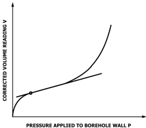
FIG. 4 Ideal Shape of the Pressuremeter Corrected Curve
