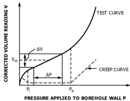
FIG. 8 Pressuremeter Test Curves for Procedure A
